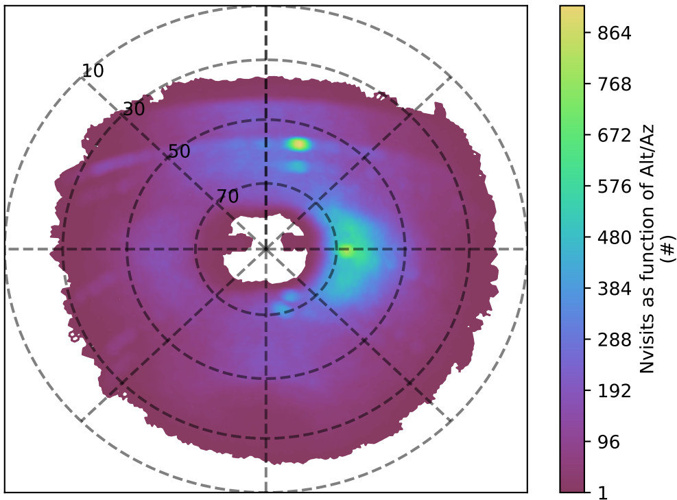
ddf_acor_sf20_lsf40_lsr50_v3.4_10yrs u band: Nvisits as function of Alt/Az
