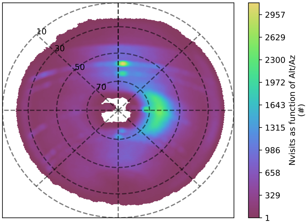
ddf_acor_sf20_lsf40_lsr50_v3.4_10yrs i band: Nvisits as function of Alt/Az
