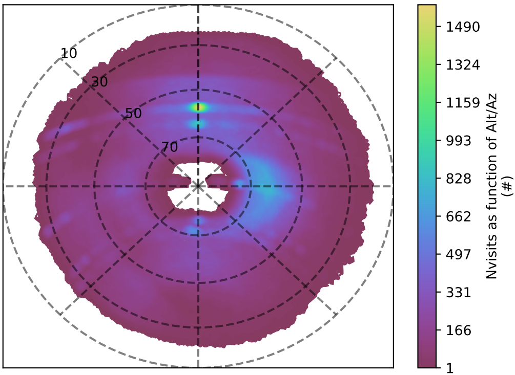
ddf_acor_sf20_lsf40_lsr50_v3.4_10yrs g band: Nvisits as function of Alt/Az
