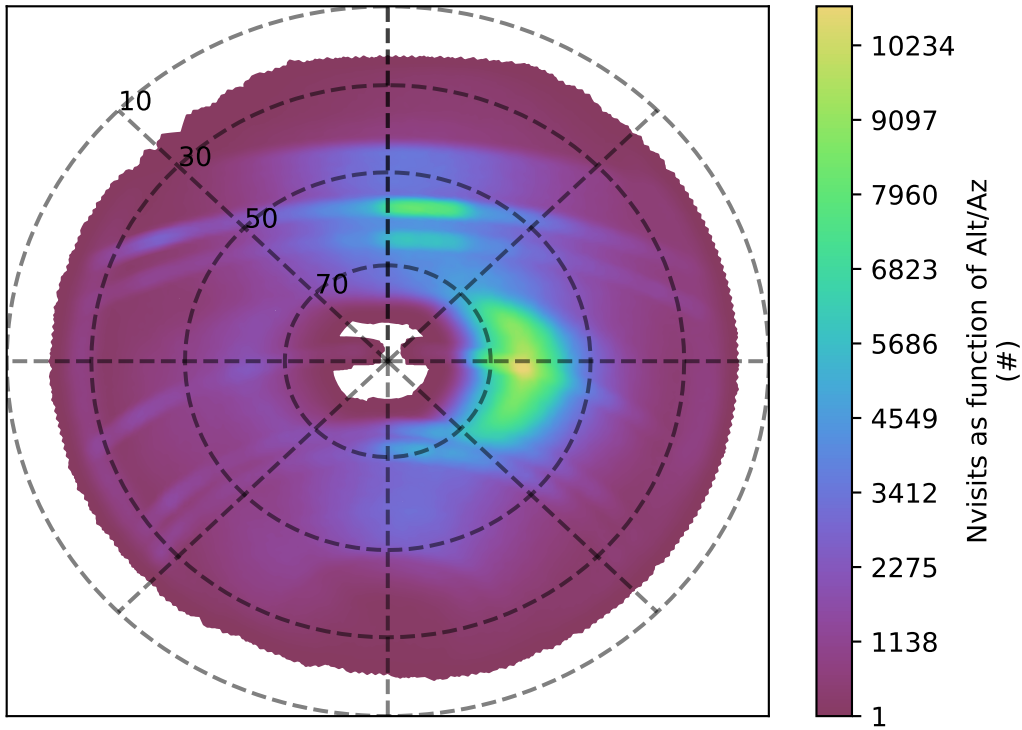
ddf_acor_sf20_ls40_lsr50_v3.4_10yrs all bands: Nvisits as function of Alt/Az
