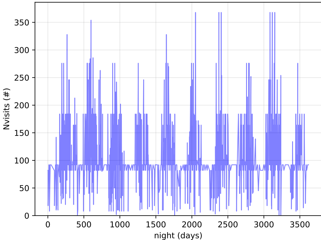
ddf_acor_sf20_ls40_lsr50_v3.4_10yrs DDF: Nvisits
