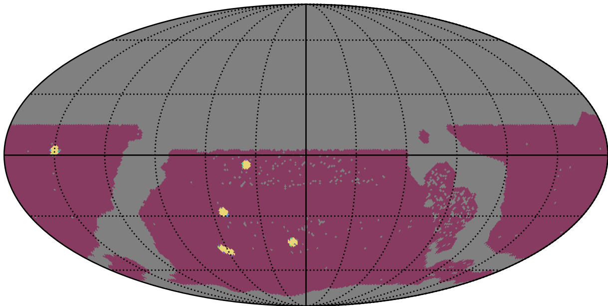
ddf_acor_sf20_lsf40_lsr50_v3.4_10yrs WFD: NumberOfQuickRevisits
