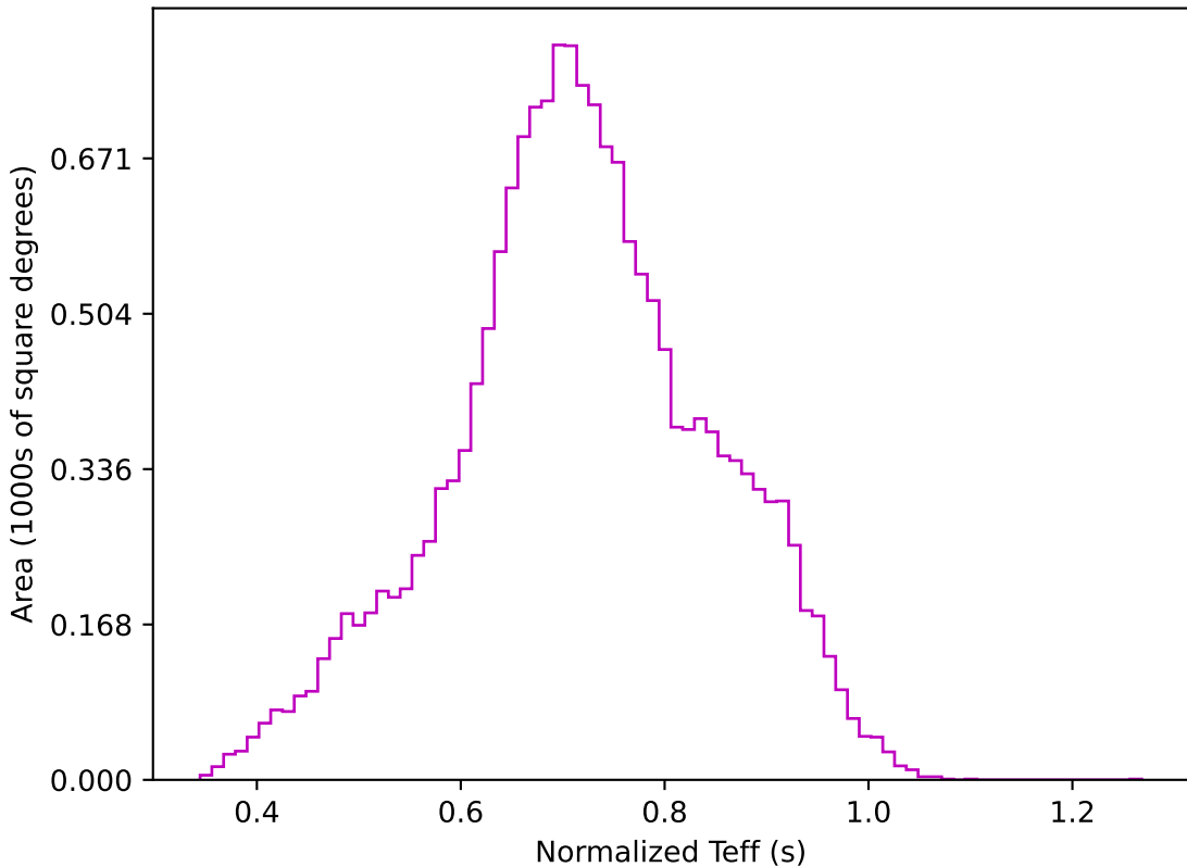
ddf_acor_sf20_lsf40_lsr50_v3.4_10yrs WFD z band: Normalized Teff
