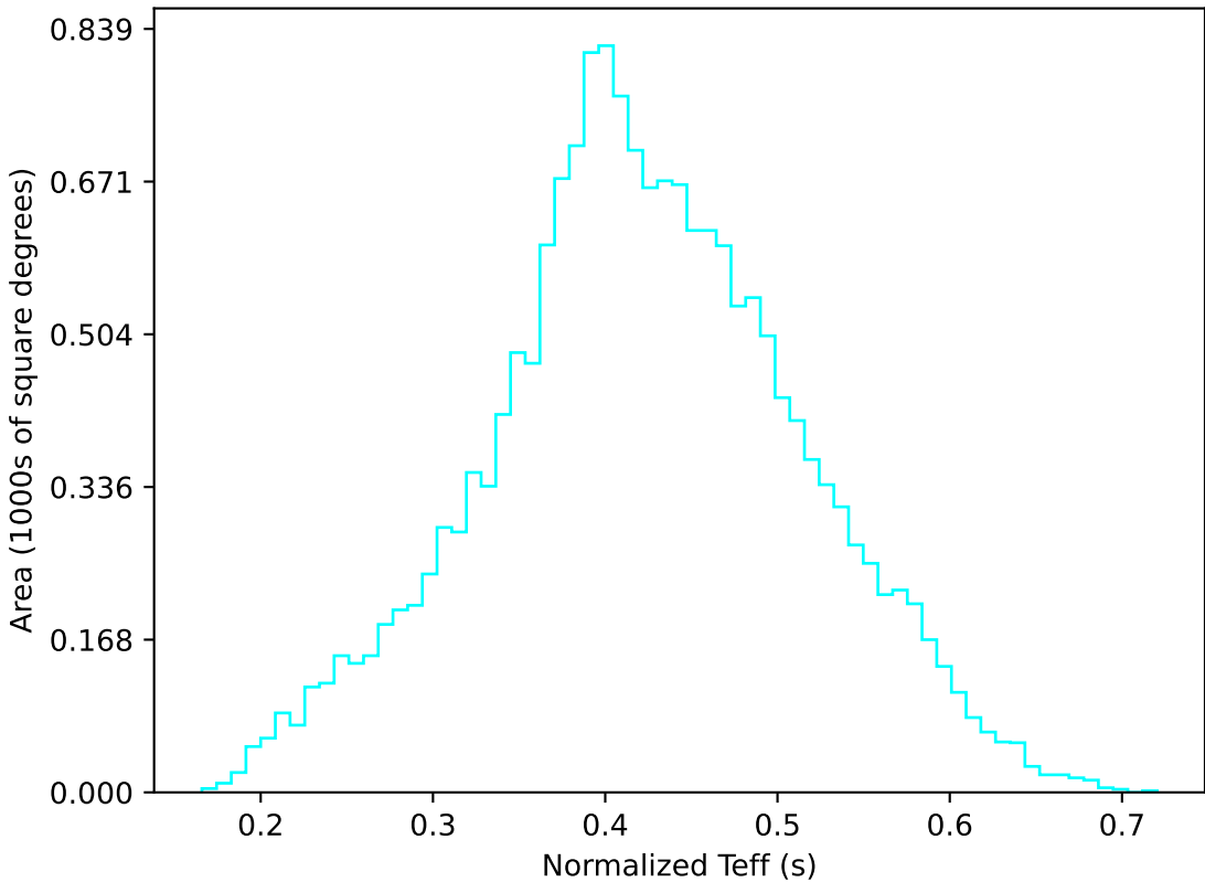
ddf_acor_sf20_lsf40_lsr50_v3.4_10yrs WFD u band: Normalized Teff
