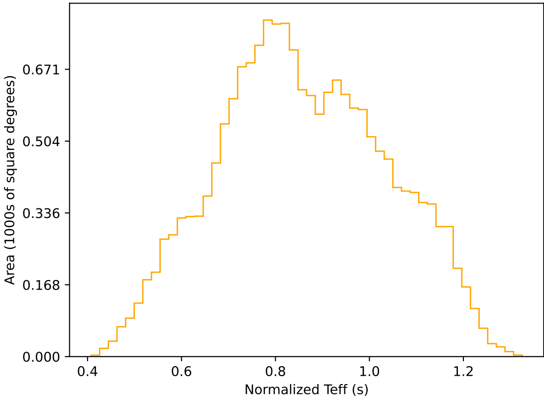
ddf_acor_sf20_lsf40_lsr50_v3.4_10yrs WFD r band: Normalized Teff
