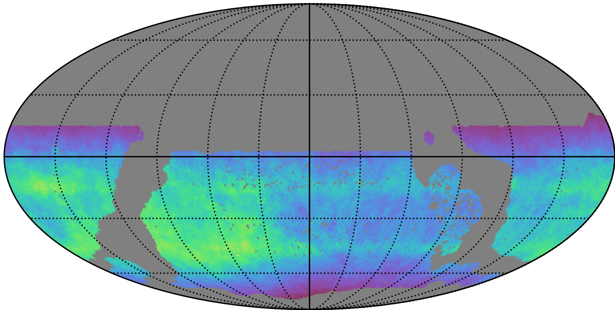
ddf_acor_sf20_lsf40_lsr50_v3.4_10yrs WFD i band: Normalized Teff
