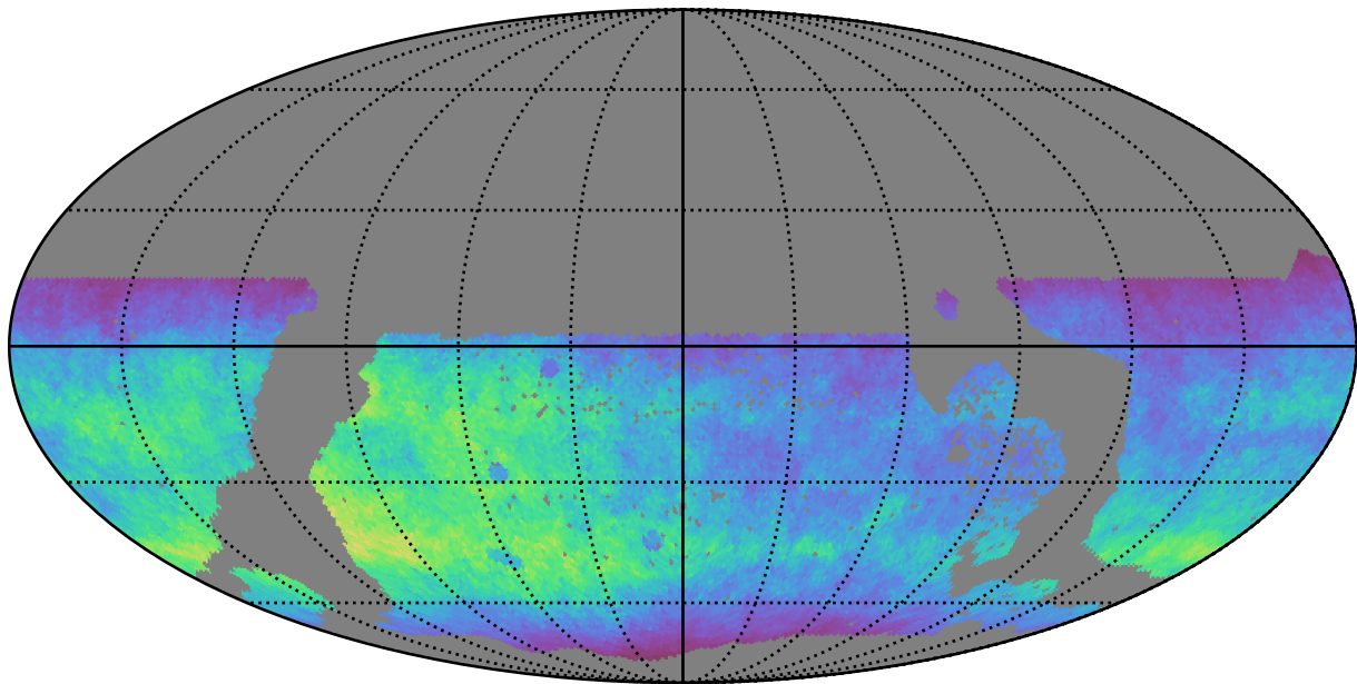
ddf_acor_sf20_lsf40_lsr50_v3.4_10yrs WFD g band: Normalized Teff
