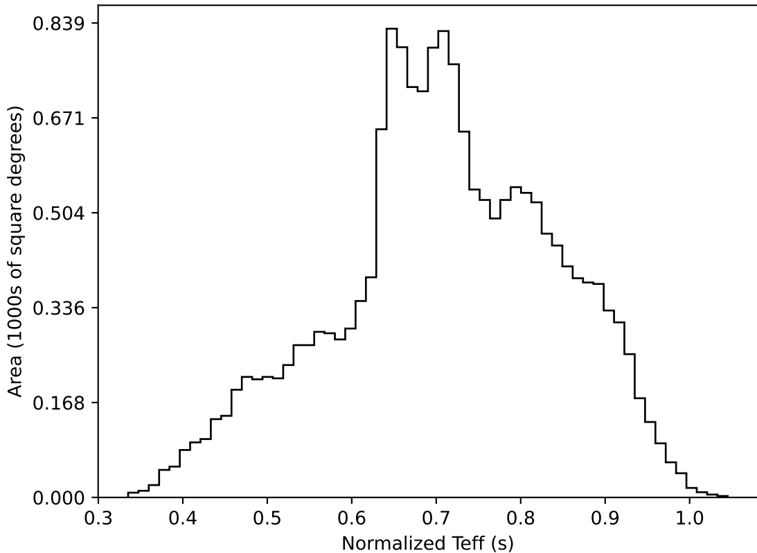
ddf_acor_sf20_lsf40_lsr50_v3.4_10yrs WFD all bands: Normalized Teff
