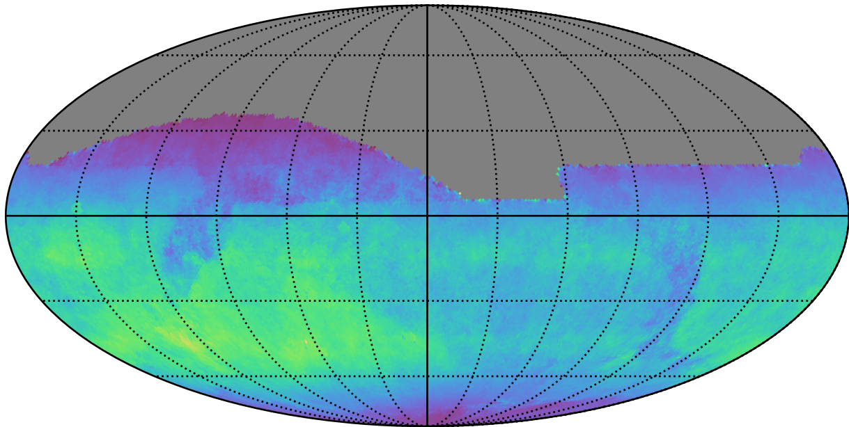
ddf_acor_sf20_lsf40_lsr50_v3.4_10yrs All sky z band: Normalized Teff
