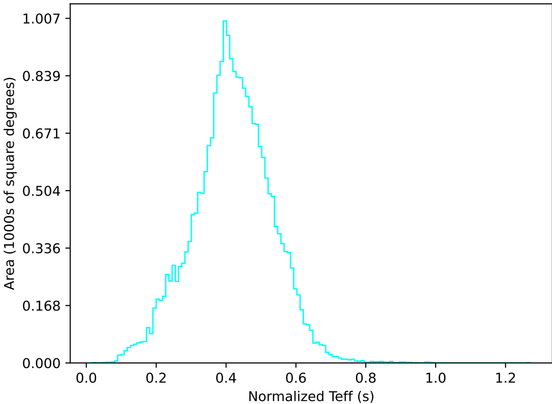
ddf_acor_sf20_lsf40_lsr50_v3.4_10yrs All sky u band: Normalized Teff
