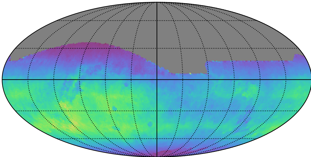
ddf_acor_sf20_lsf40_lsr50_v3.4_10yrs All sky r band: Normalized Teff
