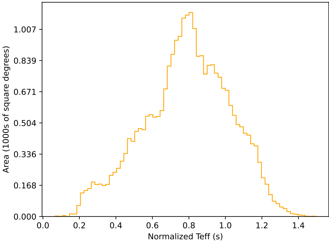
ddf_acor_sf20_lsf40_lsr50_v3.4_10yrs All sky r band: Normalized Teff
