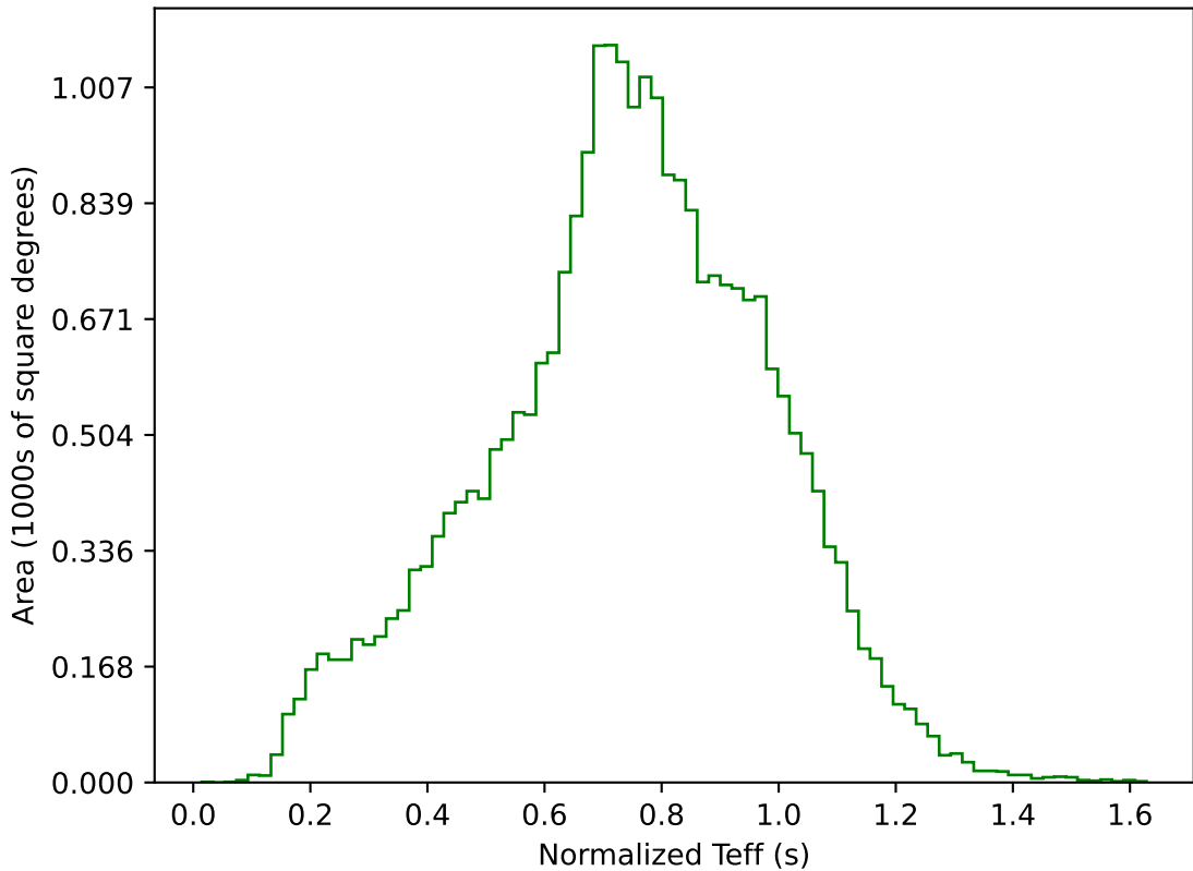
ddf_acor_sf20_lsf40_lsr50_v3.4_10yrs All sky g band: Normalized Teff
