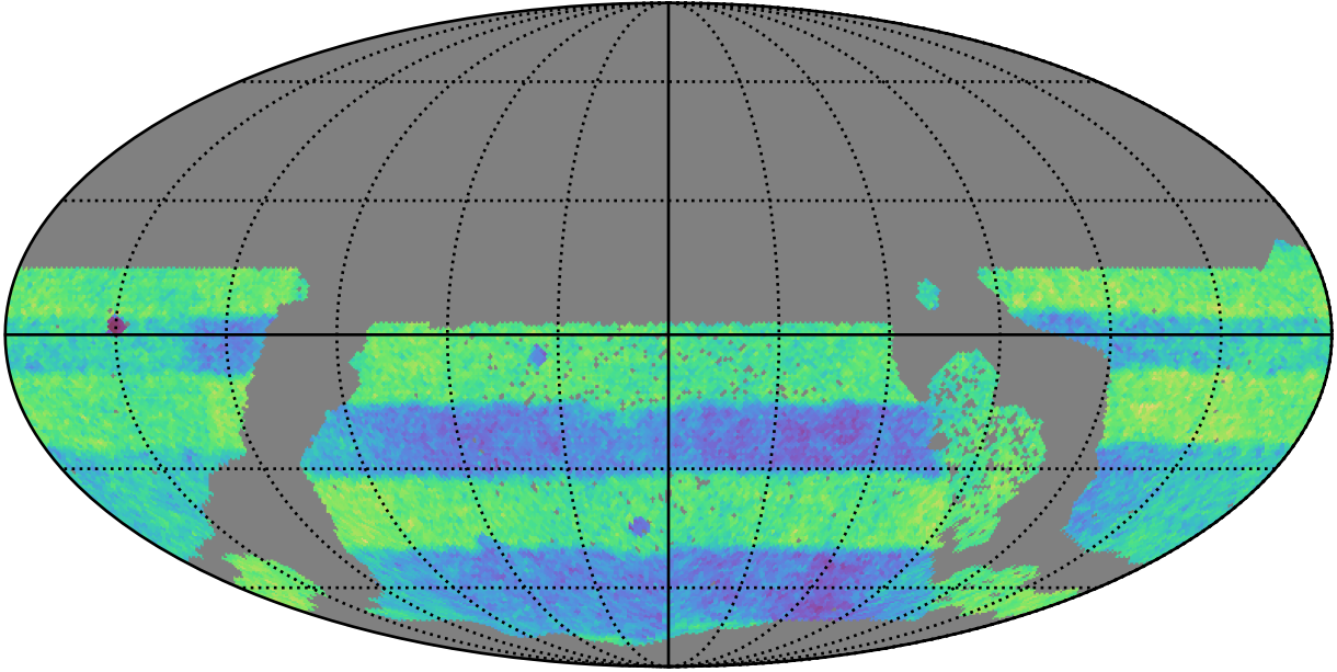
ddf_acor_sf20_lsf40_lsr50_v3.4_10yrs WFD: Normalized Proper Motion Uncert @ 20.5
