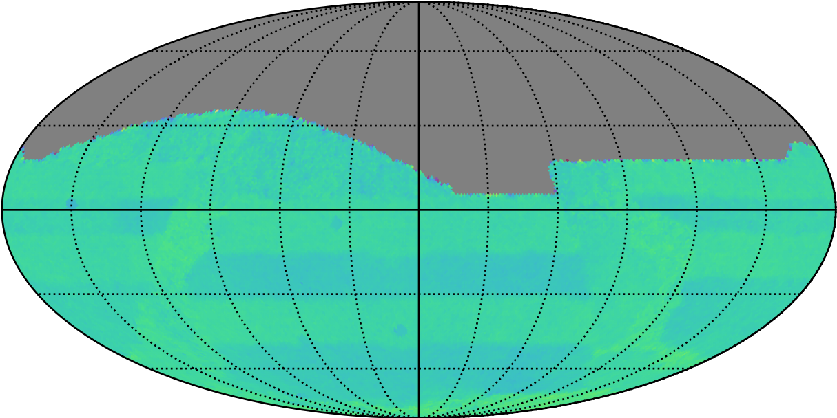
ddf_acor_sf20_lsf40_lsr50_v3.4_10yrs All sky: Normalized Proper Motion Uncert @ 20.5
