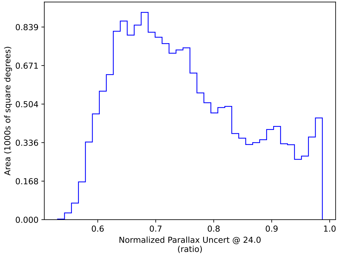
ddf_acor_sf20_lsf40_lsr50_v3.4_10yrs WFD: Normalized Parallax Uncert @ 24.0
