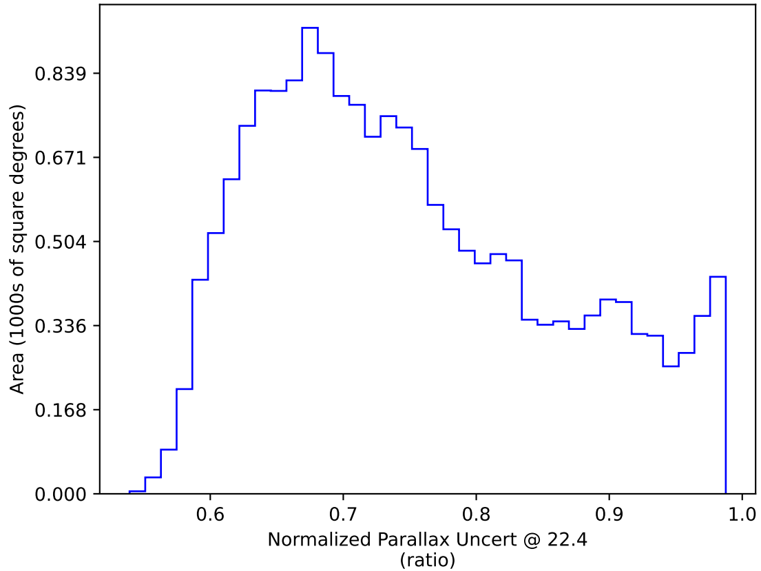
ddf_acor_sf20_lsf40_lsr50_v3.4_10yrs WFD: Normalized Parallax Uncert @ 22.4
