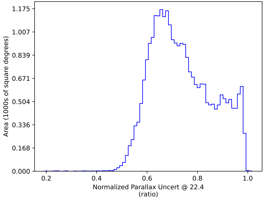
ddf_acor_sf20_lsf40_lsr50_v3.4_10yrs All sky: Normalized Parallax Uncert @ 22.4
