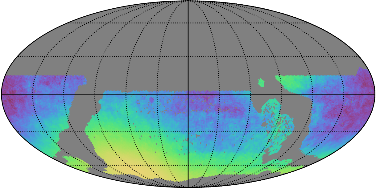
ddf_acor_sf20_lsf40_lsr50_v3.4_10yrs WFD y band only: Normalized Parallax Uncert @ 21.3
