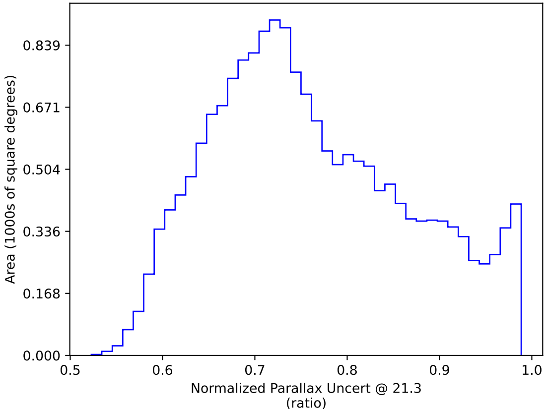
ddf_acor_sf20_lsf40_lsr50_v3.4_10yrs WFD y band only: Normalized Parallax Uncert @ 21.3
