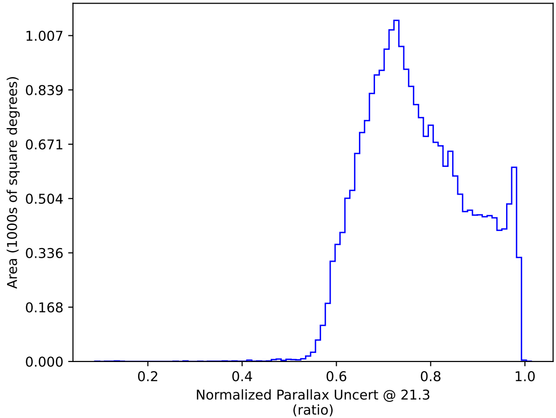
ddf_acor_sf20_lsf40_lsr50_v3.4_10yrs All sky y band only: Normalized Parallax Uncert @ 21.3
