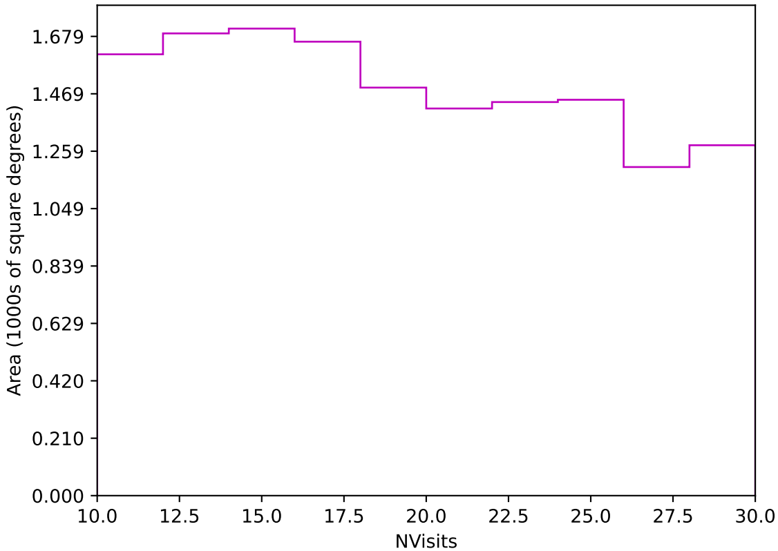
ddf_acor_sf20_lsf40_lsr50_v3.4_10yrs Yr 3-4 z band: NVisits
