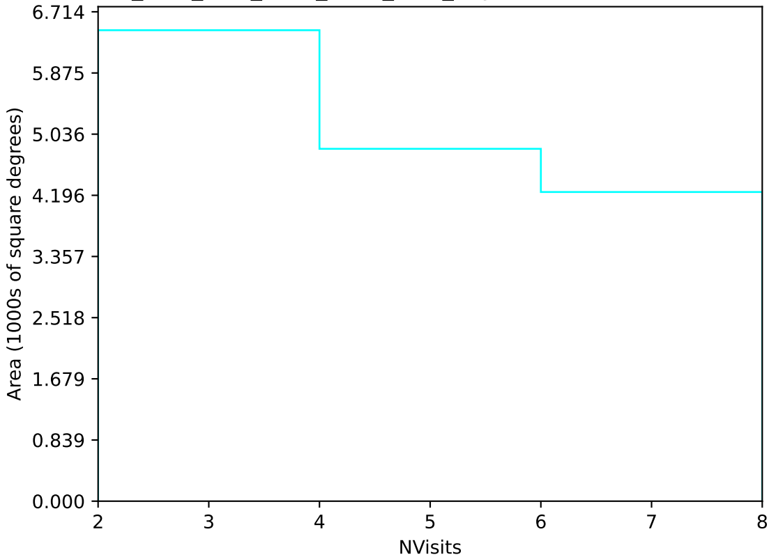
ddf_acor_sf20_lsf40_lsr50_v3.4_10yrs Yr 3-4 u band: NVisits
