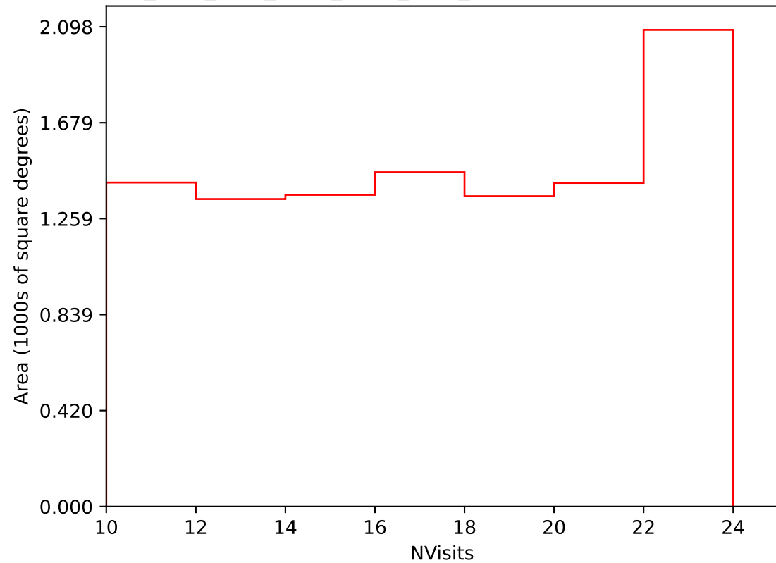
ddf_acor_sf20_lsf40_lsr50_v3.4_10yrs Yr 3-4 i band: NVisits
