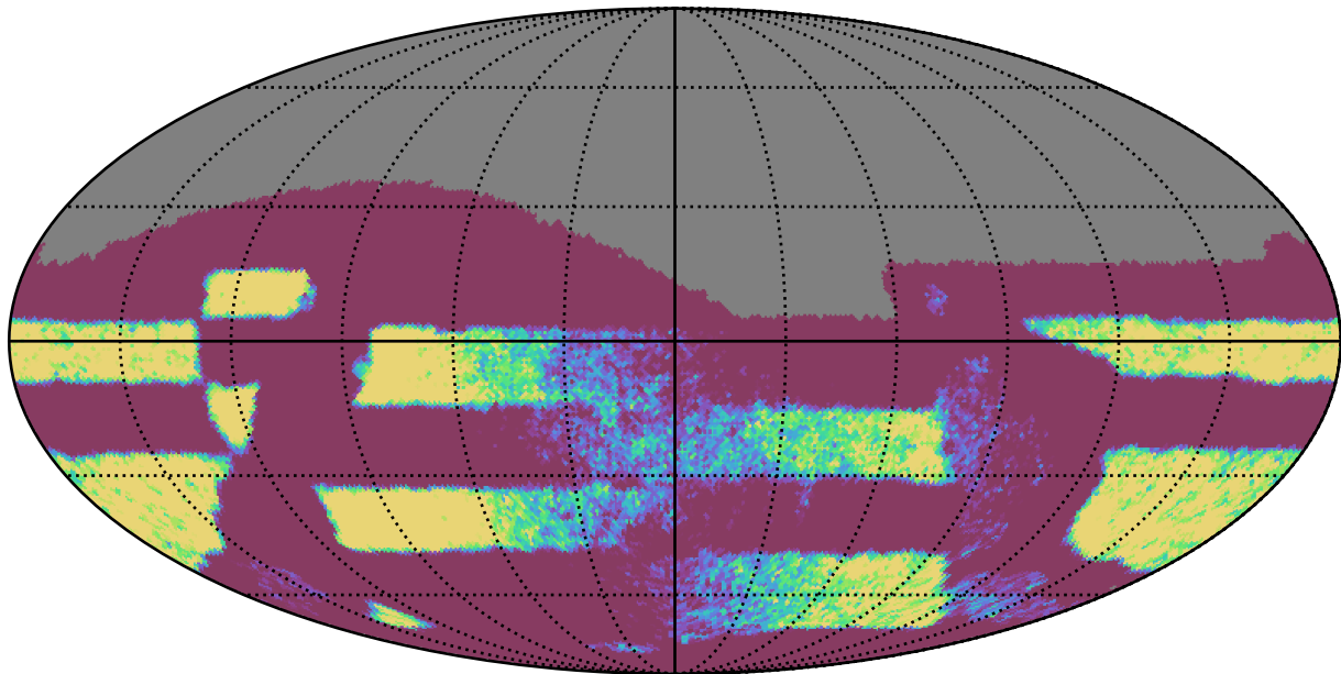
ddf_acor_sf20_lsf40_lsr50_v3.4_10yrs Yr 3-4 all bands: NVisits
