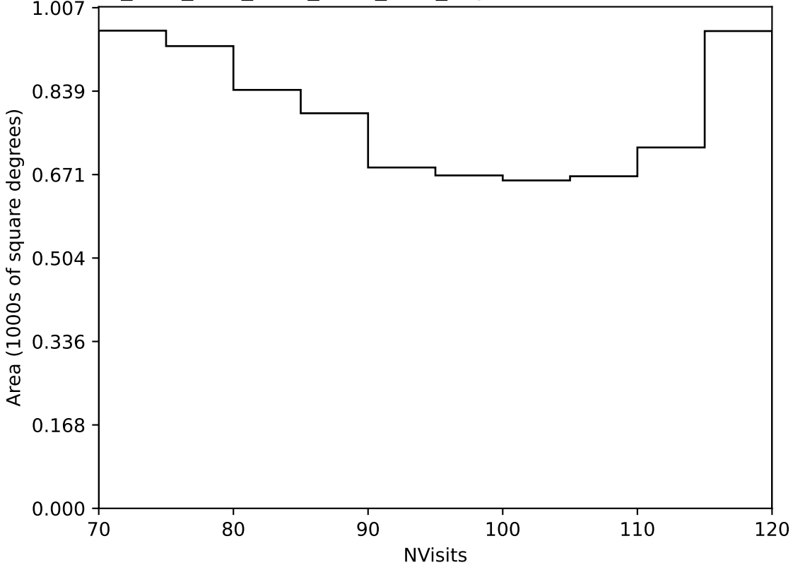
ddf_acor_sf20_lsf40_lsr50_v3.4_10yrs Yr 3-4 all bands: NVisits
