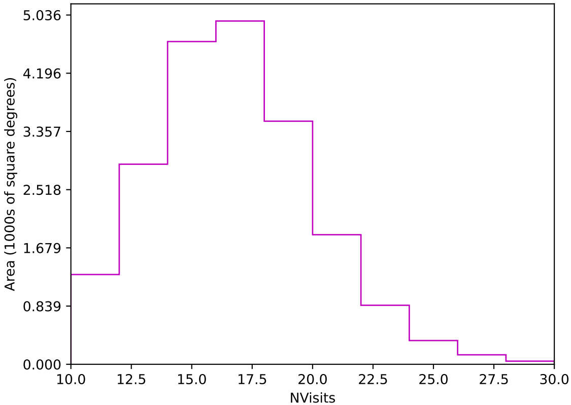
ddf_acor_sf20_lsf40_lsr50_v3.4_10yrs Yr 1 z band: NVisits
