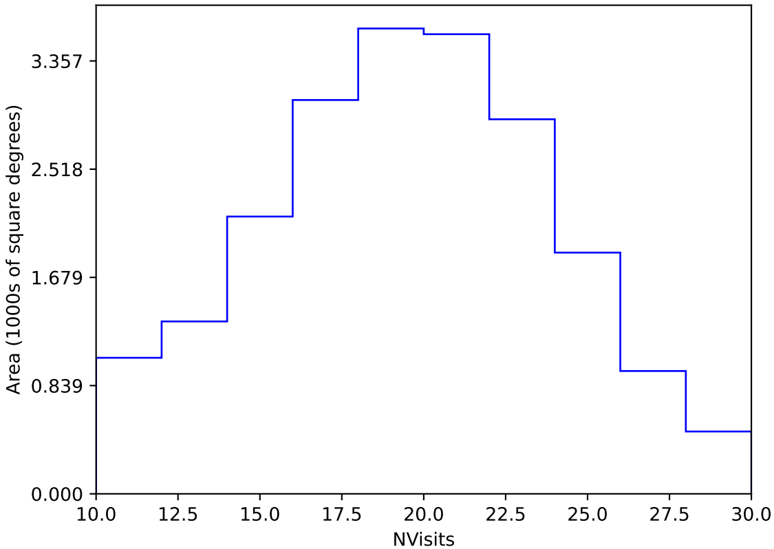
ddf_acor_sf20_lsf40_lsr50_v3.4_10yrs Yr 1 y band: NVisits
