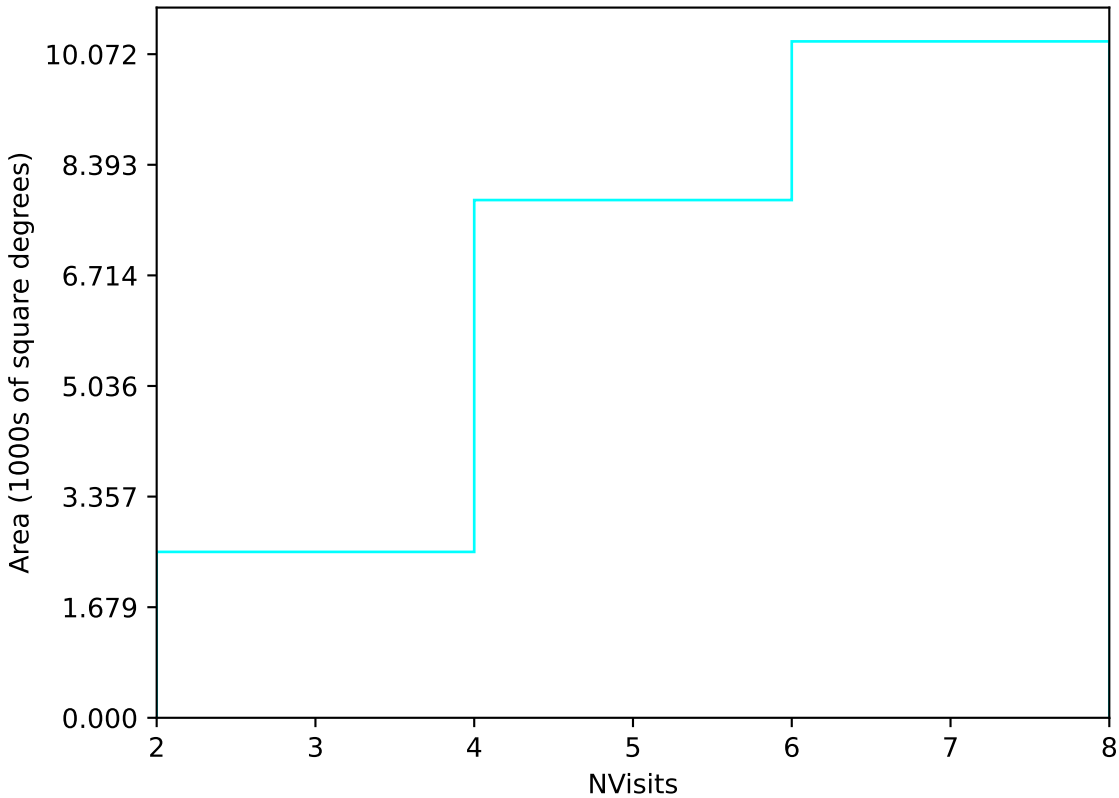
ddf_acor_sf20_lsf40_lsr50_v3.4_10yrs Yr 1 u band: NVisits
