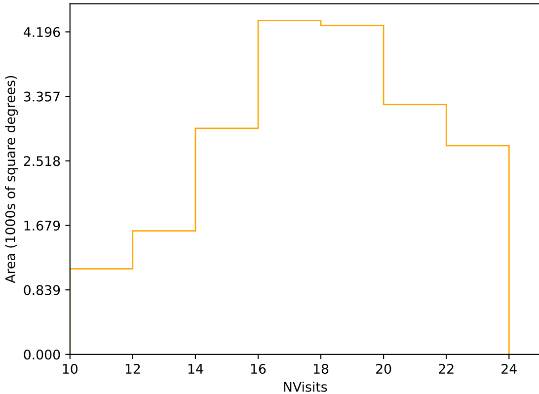
ddf_acor_sf20_lsf40_lsr50_v3.4_10yrs Yr 1 r band: NVisits
