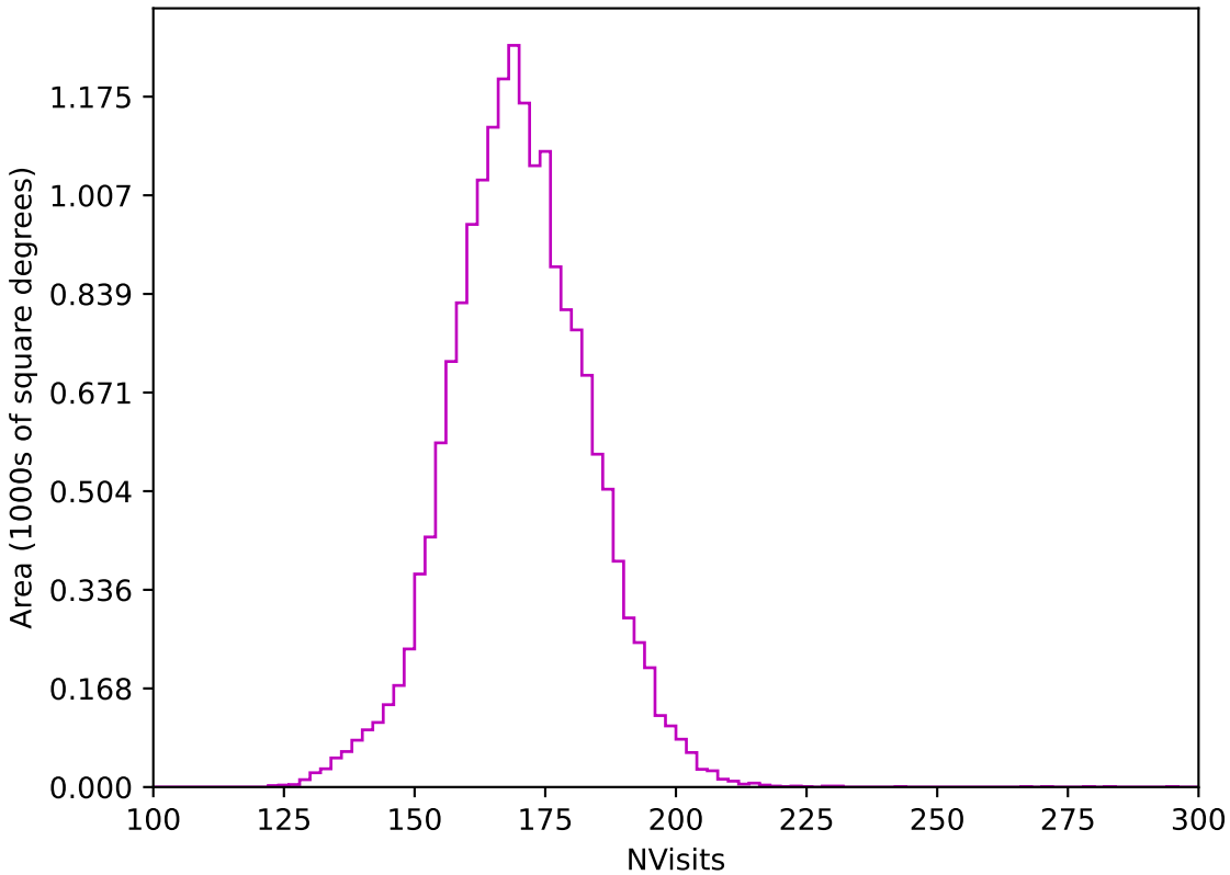
ddf_acor_sf20_lsf40_lsr50_v3.4_10yrs WFD z band: NVisits
