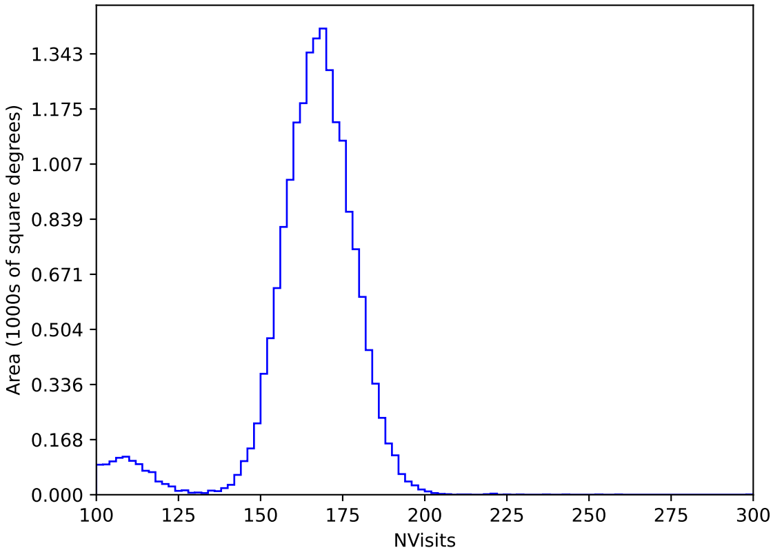
ddf_acor_sf20_lsf40_lsr50_v3.4_10yrs WFD y band: NVisits
