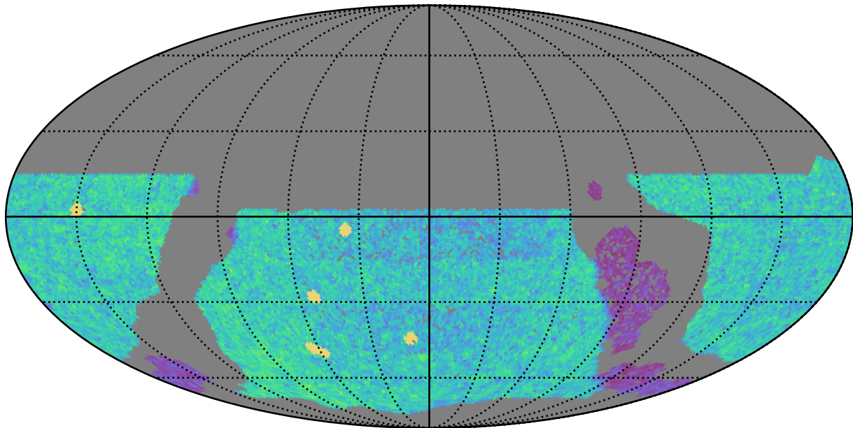
ddf_acor_sf20_lsf40_lsr50_v3.4_10yrs WFD u band: NVisits
