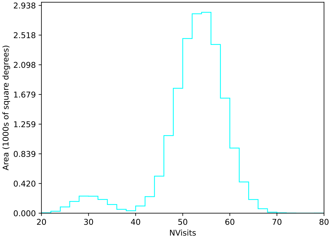
ddf_acor_sf20_lsf40_lsr50_v3.4_10yrs WFD u band: NVisits
