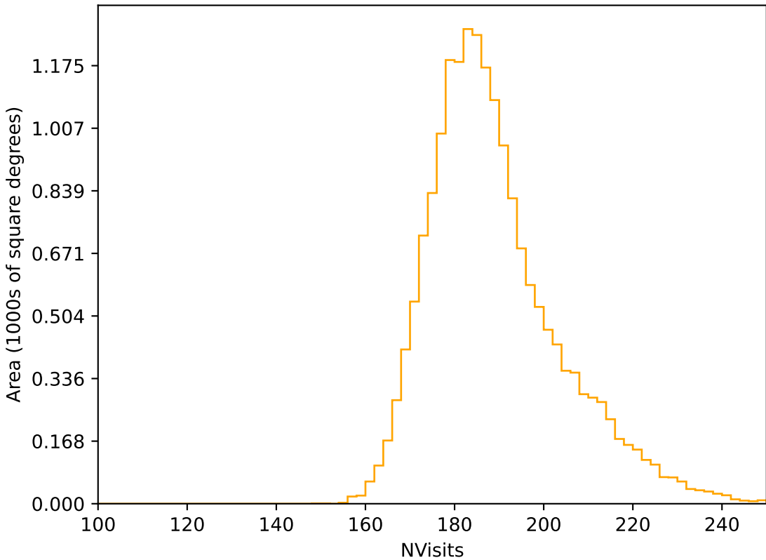
ddf_acor_sf20_lsf40_lsr50_v3.4_10yrs WFD r band: NVisits
