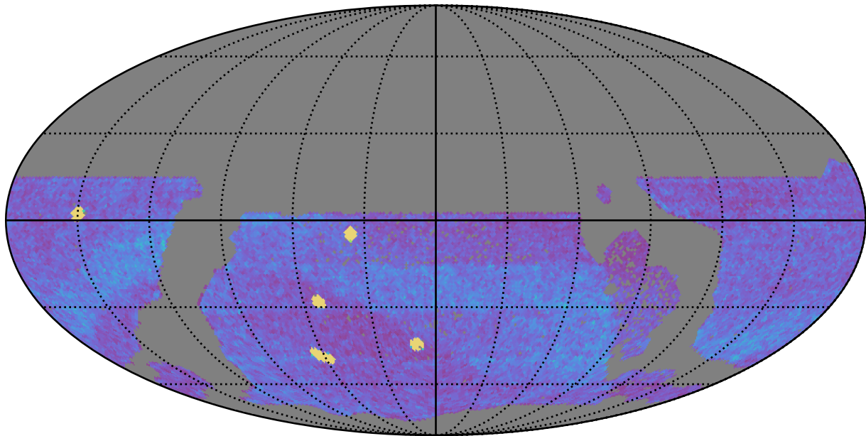
ddf_acor_sf20_lsf40_lsr50_v3.4_10yrs WFD all bands: NVisits
