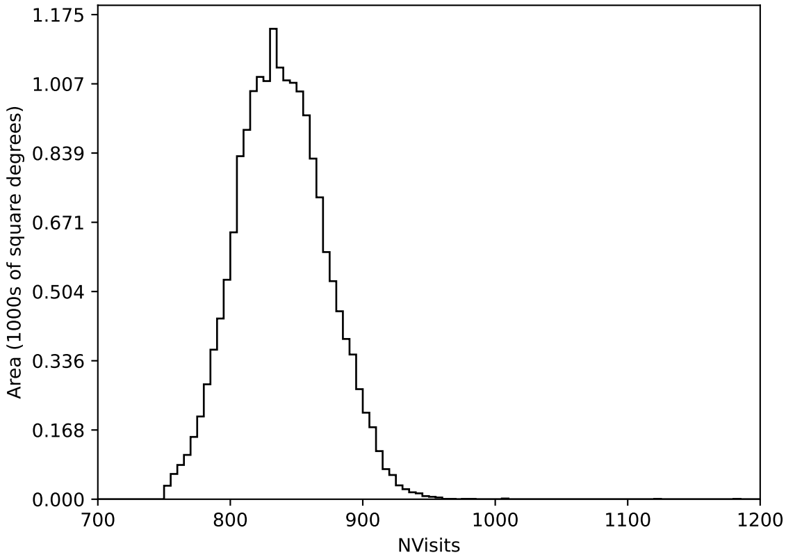
ddf_acor_sf20_lsf40_lsr50_v3.4_10yrs WFD all bands: NVisits
