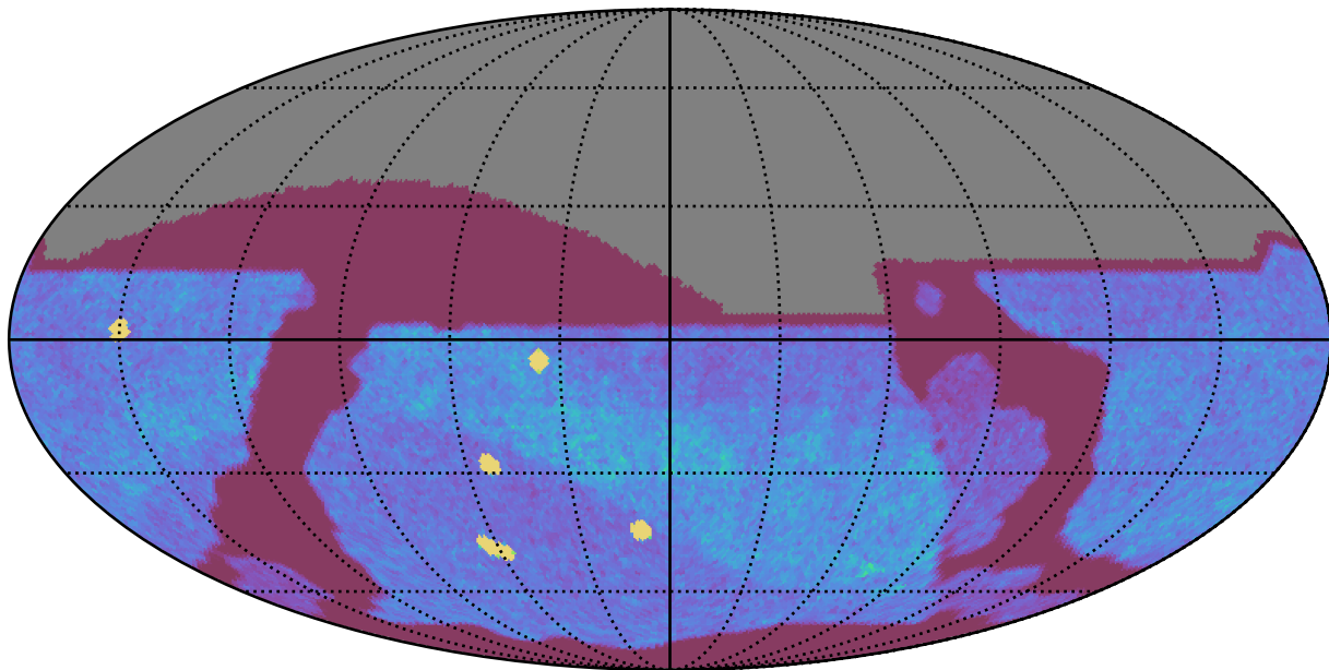
ddf_acor_sf20_lsf40_lsr50_v3.4_10yrs All sky z band: NVisits
