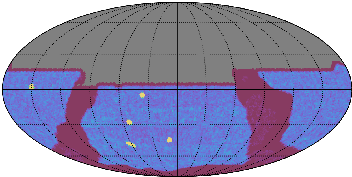
ddf_acor_sf20_lsf40_lsr50_v3.4_10yrs All sky y band: NVisits
