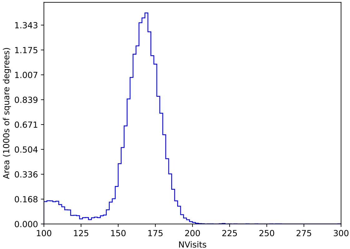
ddf_acor_sf20_lsf40_lsr50_v3.4_10yrs All sky y band: NVisits
