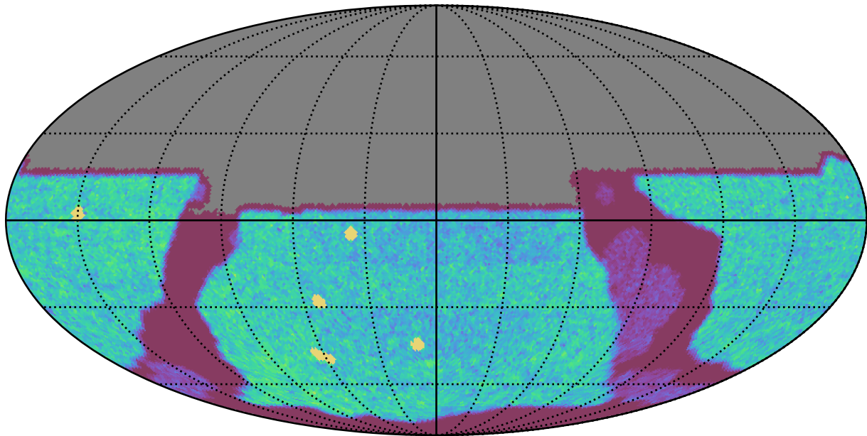
ddf_acor_sf20_lsf40_lsr50_v3.4_10yrs All sky u band: NVisits
