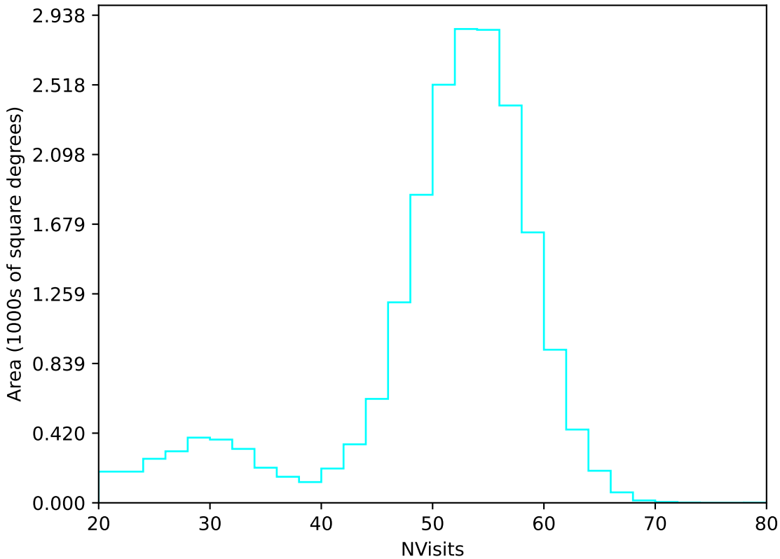
ddf_acor_sf20_lsf40_lsr50_v3.4_10yrs All sky u band: NVisits
