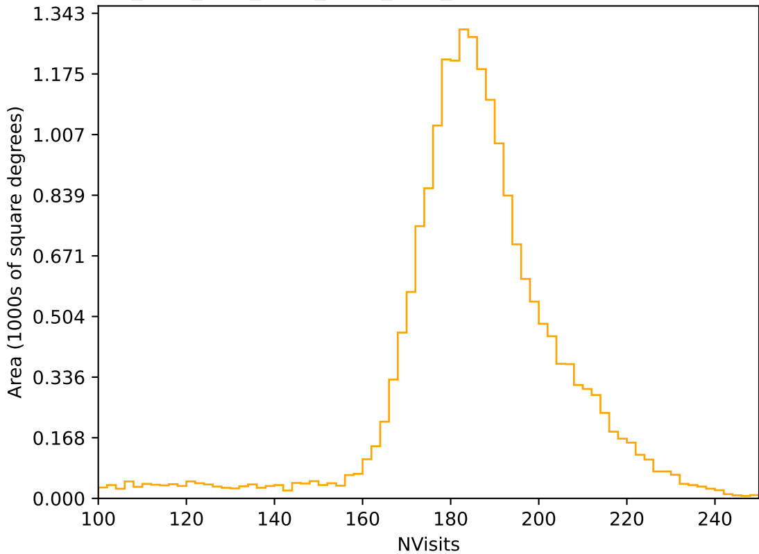
ddf_acor_sf20_lsf40_lsr50_v3.4_10yrs All sky r band: NVisits
