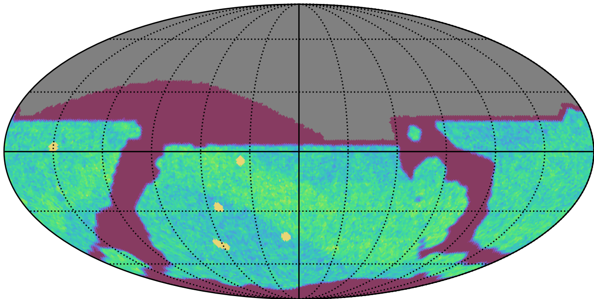
ddf_acor_sf20_lsf40_lsr50_v3.4_10yrs All sky i band: NVisits
