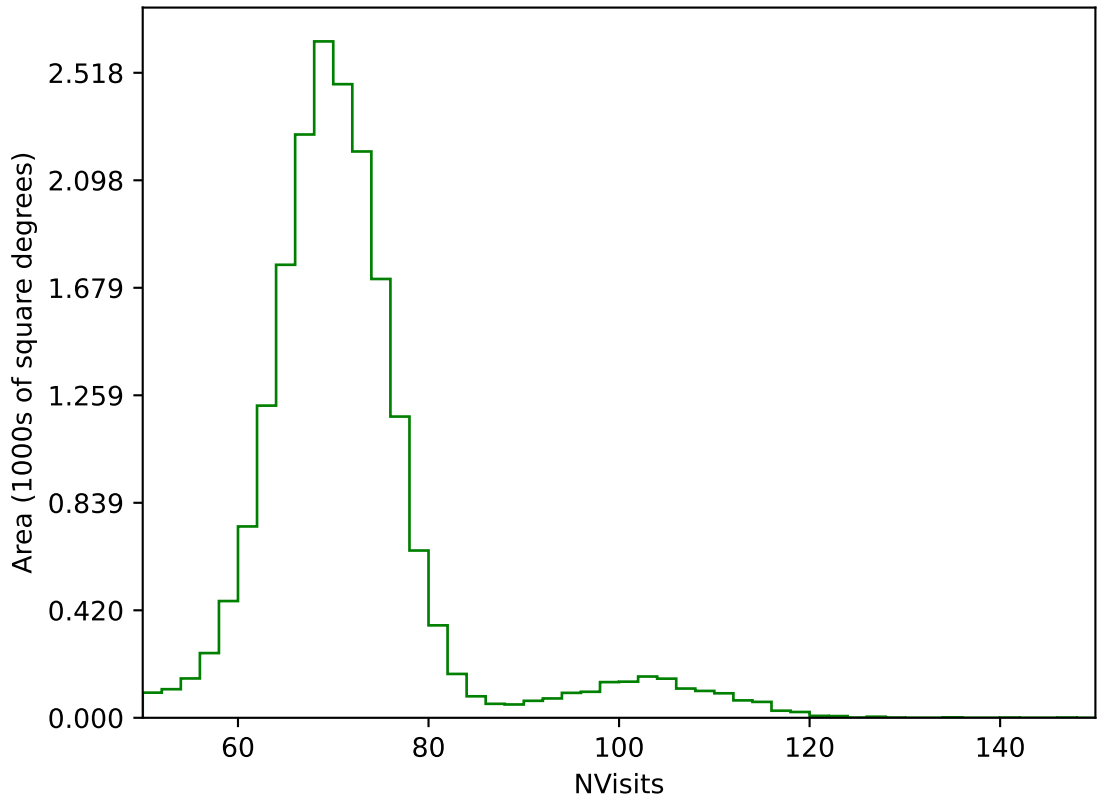
ddf_acor_sf20_lsf40_lsr50_v3.4_10yrs All sky g band: NVisits
