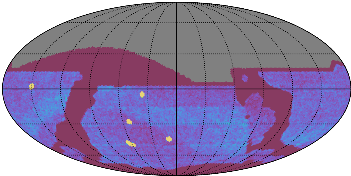
ddf_acor_sf20_lsf40_lsr50_v3.4_10yrs All sky all bands: NVisits
